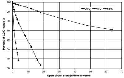
Figure 3: ODYSSEY™ Battery storage time at temperatures
